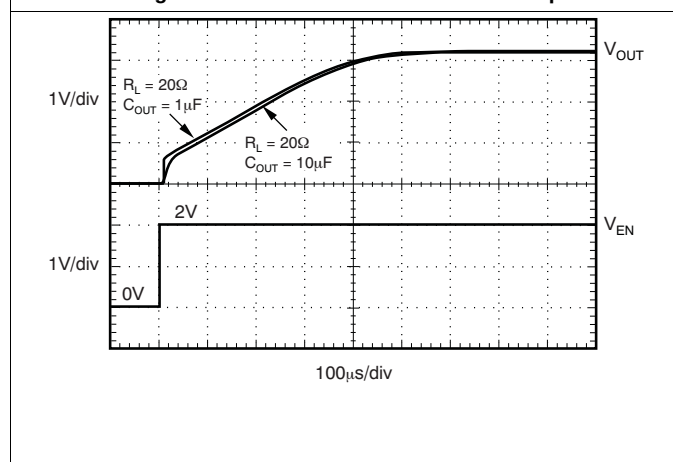
Figure 21. TPS73701 Turnon Response
