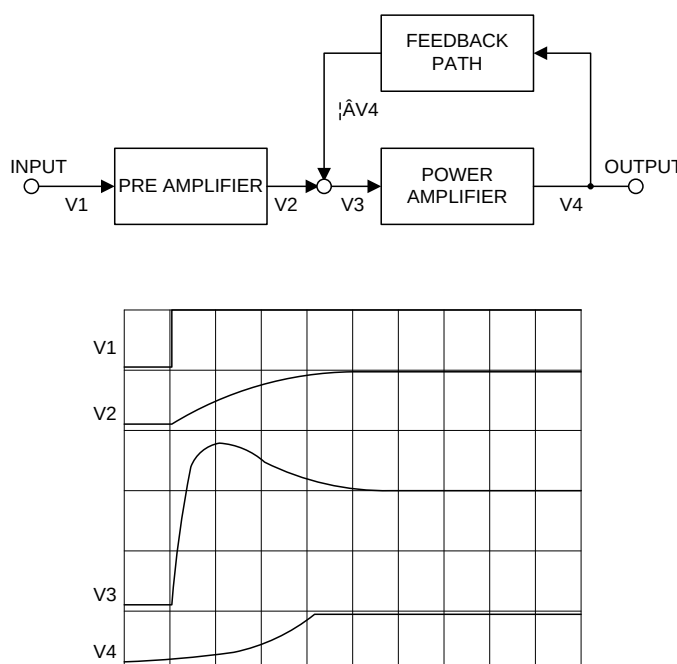
Fig.5 Overshoot phenomenon in feedback amplifiers
