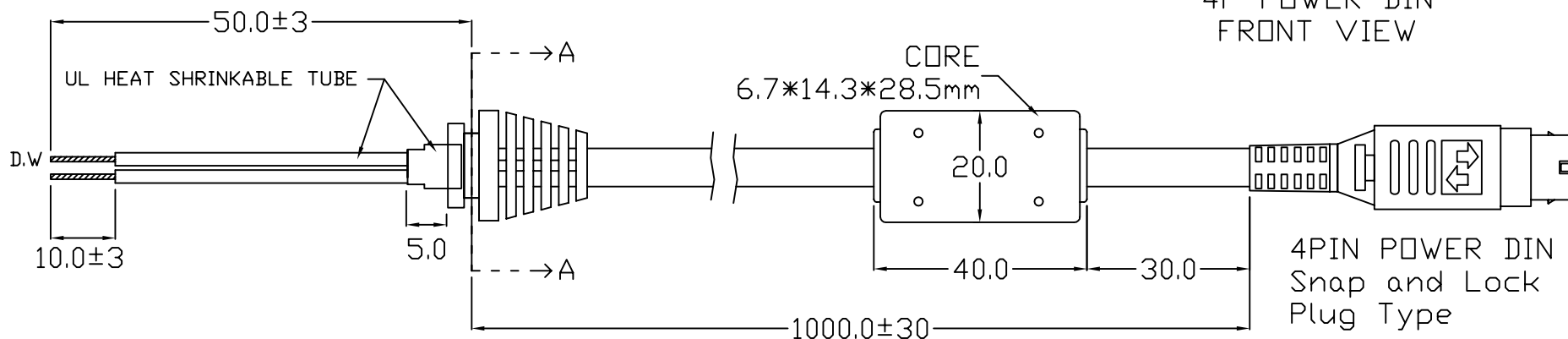
[1571#14AWG 1C+1] SECTIONAL DRAWING
