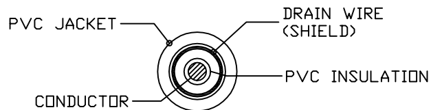
[1571#14AWG 1C+1] SECTIONAL DRAWING
