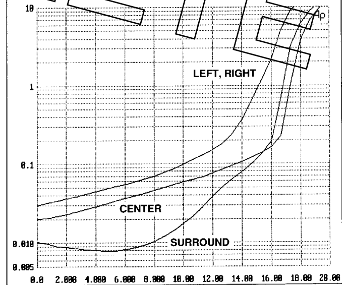
SSM-2125/2126 : Headroom THD+N(%) vs AMPL(dBr)
