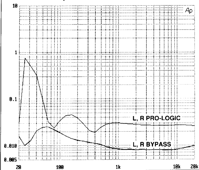
SSM-2125/2126 : Left, Right Distortion 22Hz-20kHz THD+N(%) vs FREQ(Hz)
