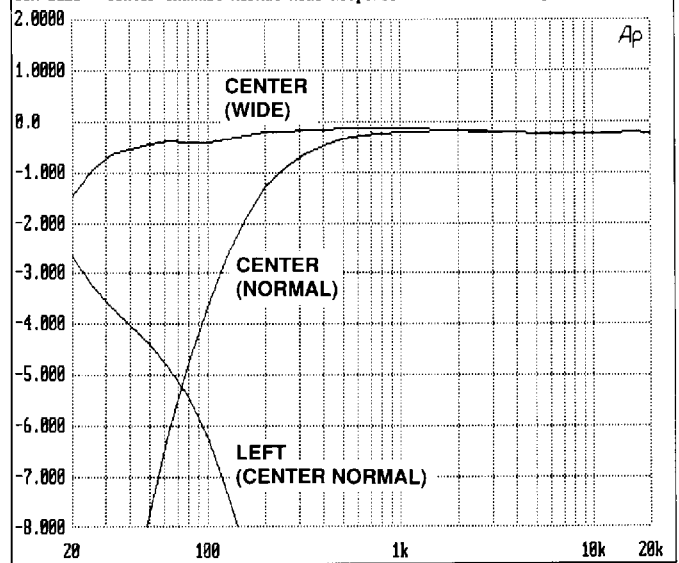
SSM-2125 : Center Channel Normal Mode Response AMPL(dBr) vs FREQ(Hz)
