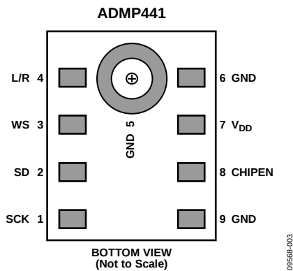
Figure 5. Pin Configuration
