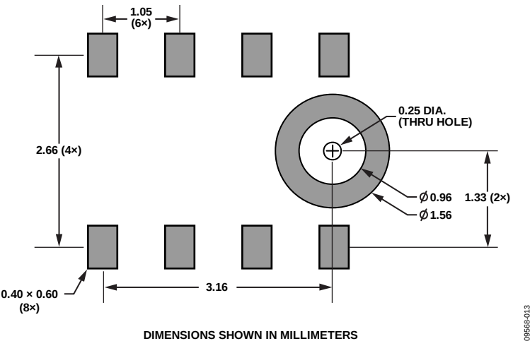
Figure 15. Recommended Printed Circuit Board Land Pattern (Dimensions shown in millimeters)
