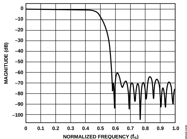
Figure 13. Digital Low-Pass Filter Magnitude Response
