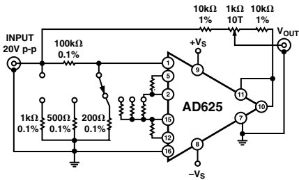
Figure 23. Settling Time Test Circuit
