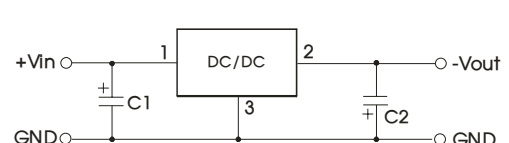
Fig. 3 Negative output application circuit
